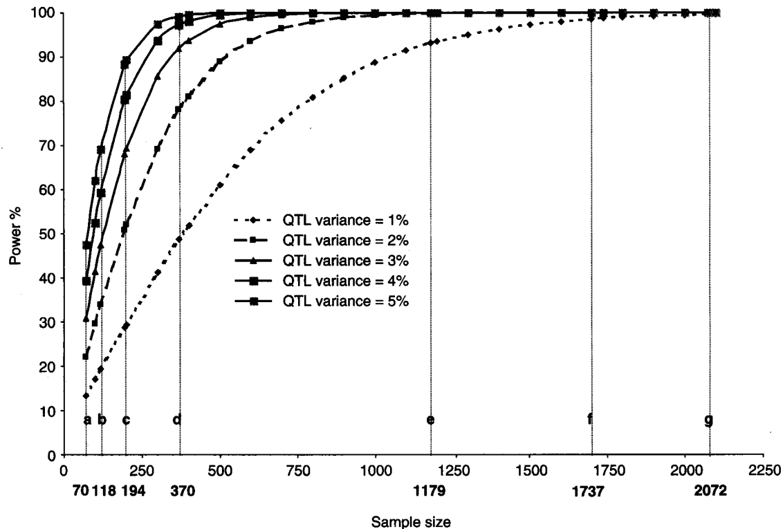
Figure 1 Power for association tests at different sample sizes to detect quantitative trait loci (QTL) explaining 1–5% of the variance ( \alpha=0.05 ). A codominant model with additive effects only (ie, dominance variance=0) is assumed. (a) Based on female subjects ( n=70 ) in Suviolahti et al. 13 (b) Based on total sample ( n=118 ) in Suviolahti et al. 13 (c) Based on total sample ( n=194 ) in Echwald et al. 11 (d) Based on total sample ( n=370 ) in Delplanque et al. 12 Based on sample size for the 8246 C/T polymorphism in the current study: (e) including one of each MZ pair, one of each DZ pair and all DZ singletons ( n=1179 ); (f) including one of each MZ pair, all DZ twins and all DZ singletons ( n=1737 ); (g) including all subjects ( n=2072 ).
